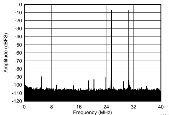
f_{IN1} = 185 \text{ MHz} , f_{IN2} = 190 \text{ MHz} , IMD3 = 89 dBFS, each tone at -7 dBFS
