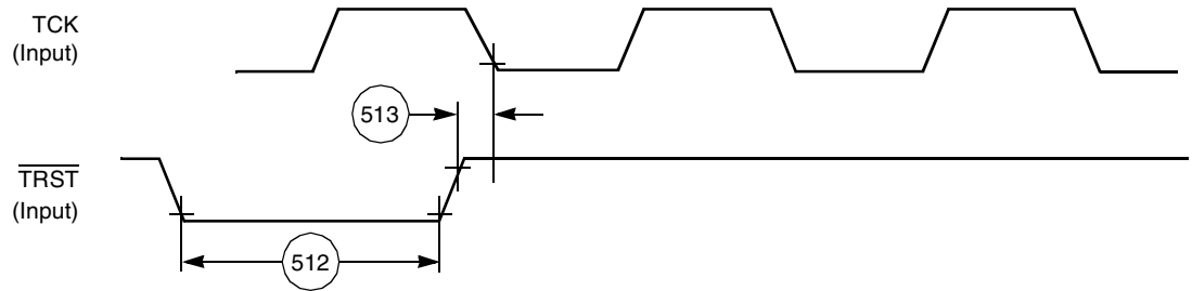
Figure 2-22. TRST Timing Diagram
