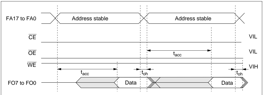
Figure 19.18 Timing Waveforms for \overline{\text{CE}}/\overline{\text{OE}} Enable State Read
