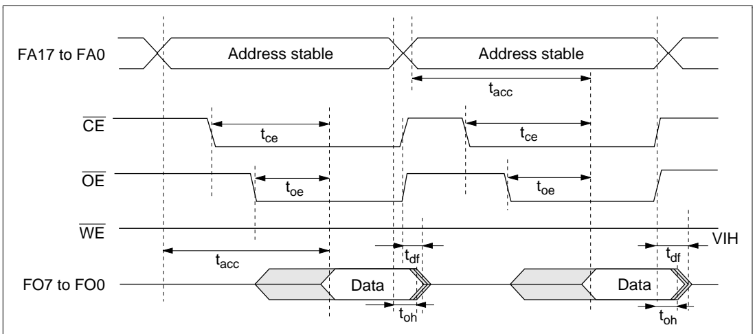
Figure 19.19 Timing Waveforms for \overline{\text{CE}}/\overline{\text{OE}} Clocked Read
