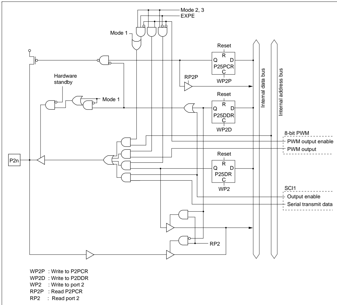
Figure C.6 Port 2 Block Diagram (Pin P25)
