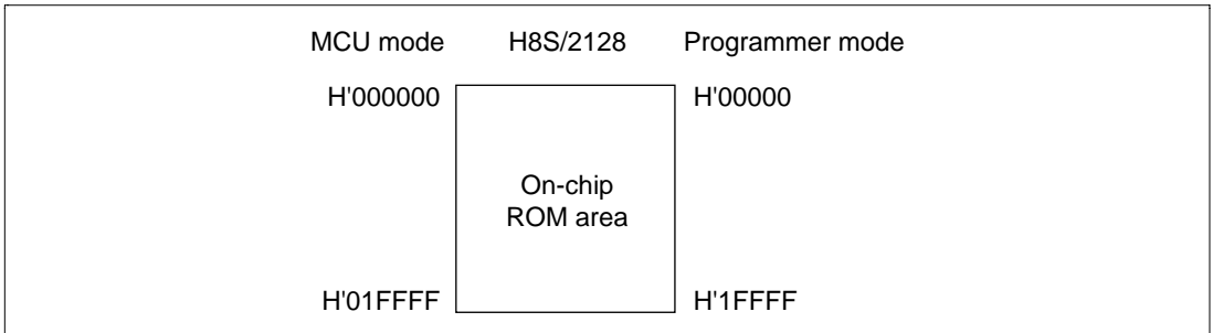
Figure 19.15 Memory Map in Programmer Mode
