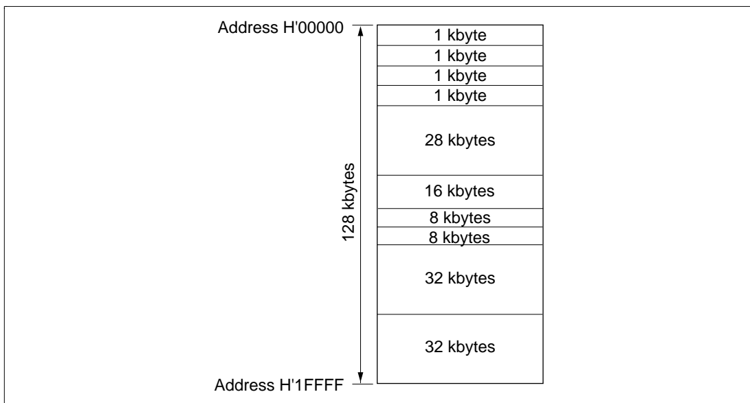
Figure 19.6 Flash Memory Block Configuration
