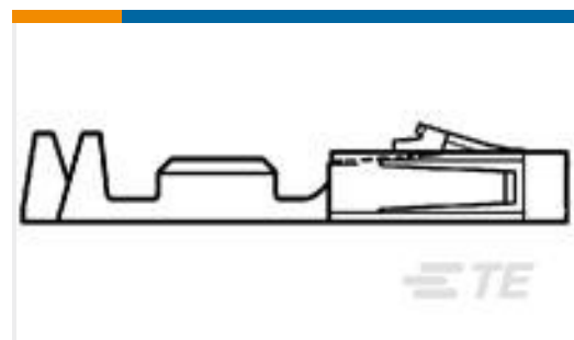
TE Part #1-104481-3 SHORT POINT RECP CONT LP
