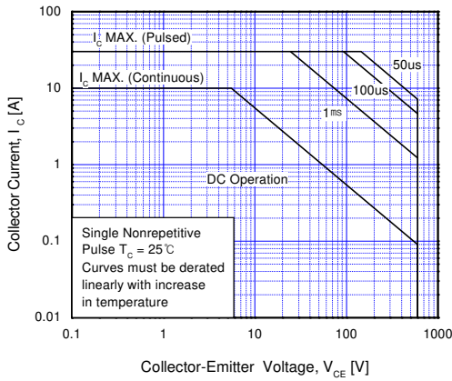
Fig 15. SOA Characteristics
