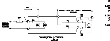
ON-OFF (FORM B) CONTROL, ACC. 49
