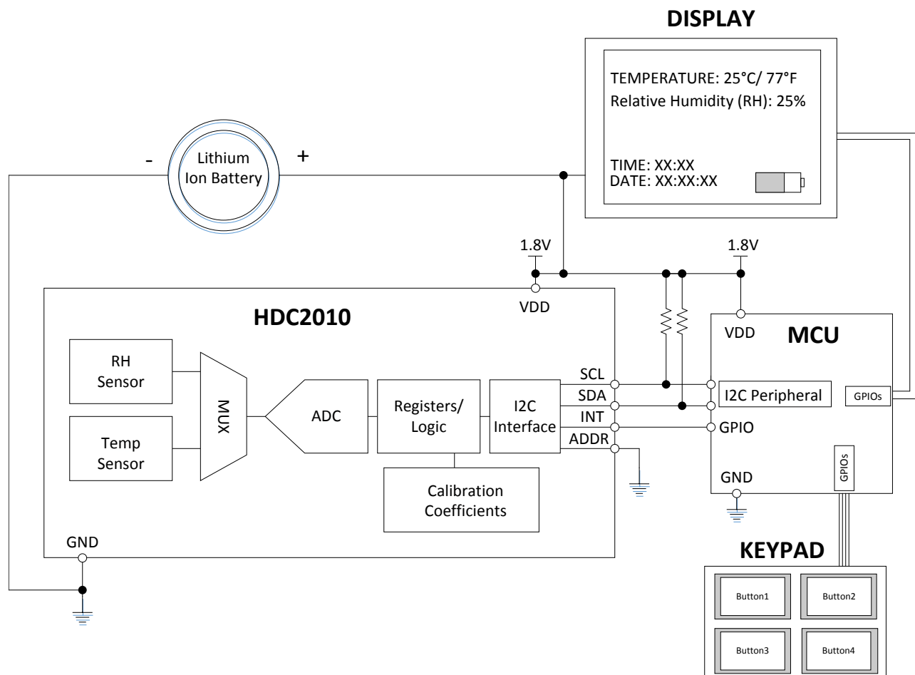
Figure 9-1. Typical Application Schematic HVAC
