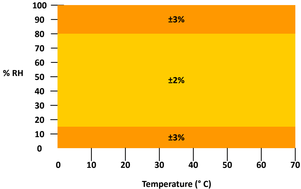
Figure 11-1. Typical Relative Humidity Accuracy Range Limits
