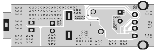
Figure 2: Top Layer
