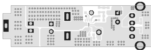
Figure 4: Bottom Layer
