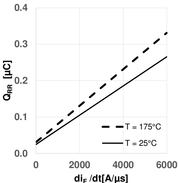
Figure 19 Typical reverse recovery charge as a function of diode current slope ( Q_{rr} = f(di_i/dt) , V_{DD} = 800V , V_{GS} = 0V/18V , I_D = 2A , ind. load, test circuit in Fig.E, body diode at V_{GS} = 0V )
