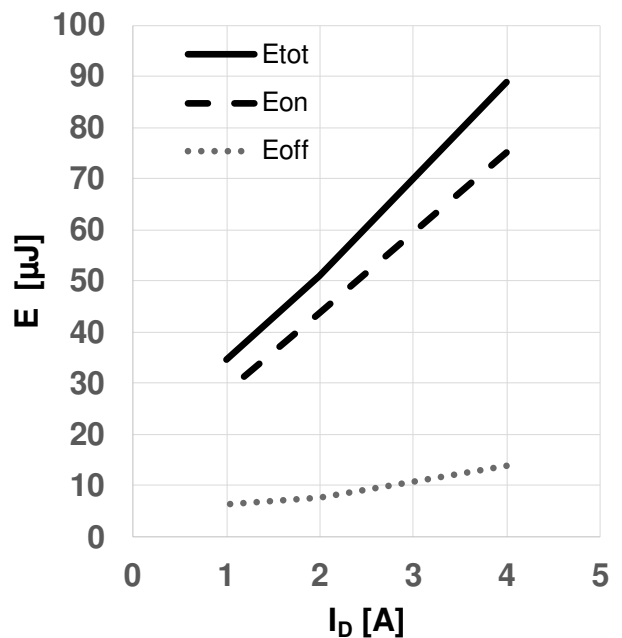
Figure 16 Typical switching energy losses as a function of drain-source current ( E = f(I_{DS}) , V_{DD} = 800\text{V} , V_{GS} = 0\text{V}/18\text{V} , R_{G,ext} = 2\Omega , T_{vj} = 175^{\circ}\text{C} , ind. load, test circuit in Fig. E, diode: body diode at V_{GS} = 0\text{V} )
