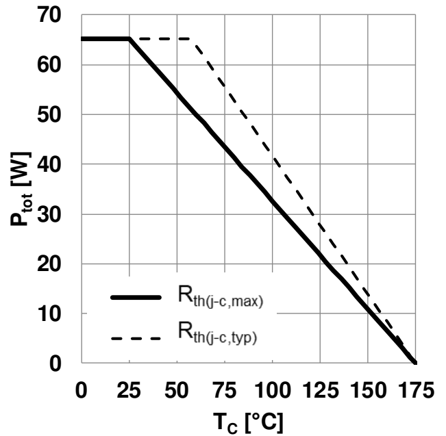
Figure 2 Power dissipation as a function of case temperature limited by bond wire temperature limited by bond wire ( P_{tot} = f(T_c) )
