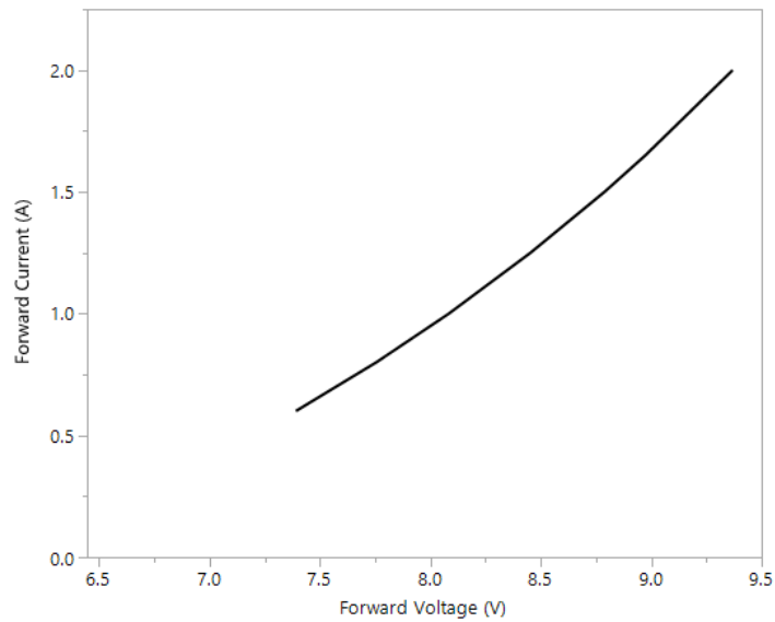
Figure 07: Forward current vs forward voltage (Measured at T_{\text{case}} = 50^\circ\text{C} )
