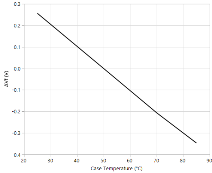
Figure 06: Normalized forward voltage vs temperature (Measured at I_f = 1.65\text{A} and normalized at T_{\text{case}} = 50^\circ\text{C} )
