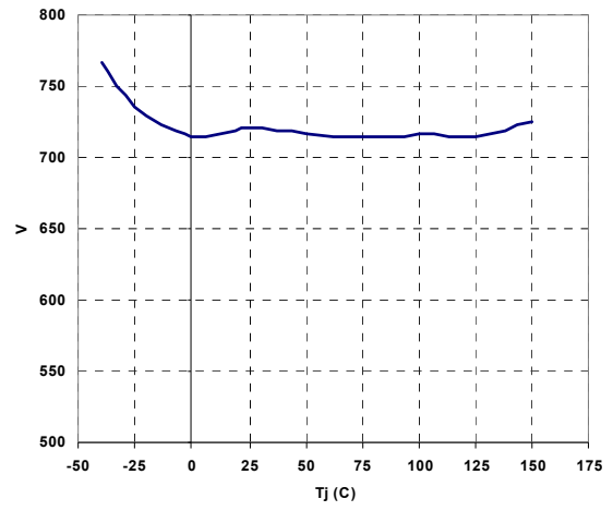
Figure 37. HV breakdown voltage vs. T_J
