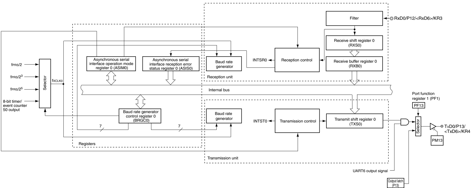
(a) 78K0/LC3
