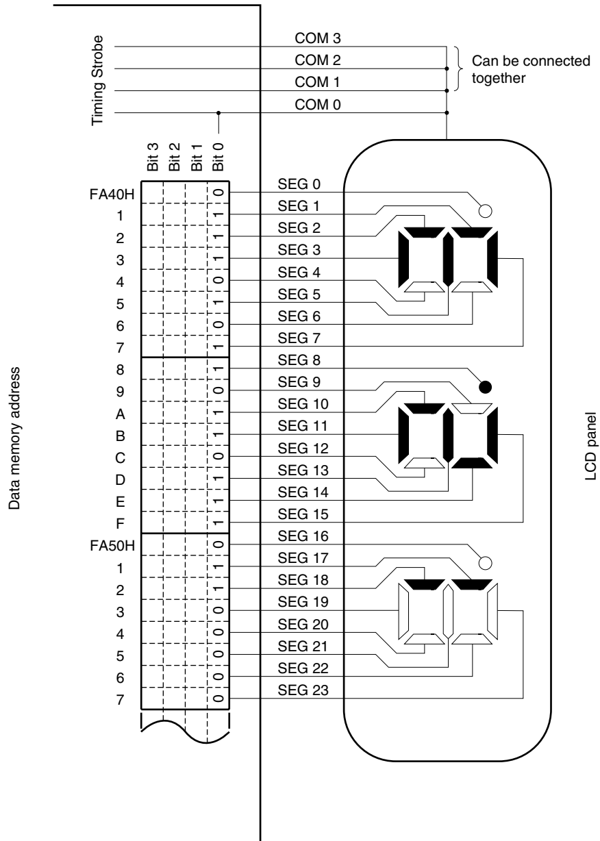
Figure 18-21. Example of Connecting Static LCD Panel
