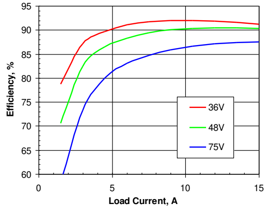
Figure 2. Efficiency vs. load current and input voltage for SSQE48T15033 converter mounted vertically with air flowing from pin 1 to pin 3 at a rate of 300 LFM (1.5 m/s) and T_a = 25^\circ C .
