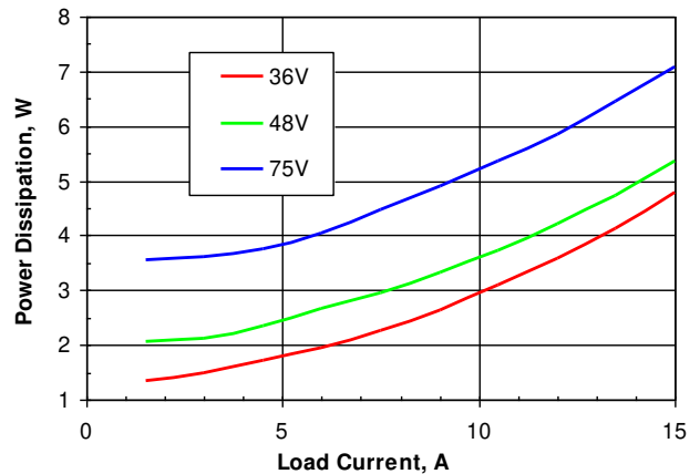
Figure 4. Power dissipation vs. load current and input voltage for SSQE48T15033 converter mounted vertically with air flowing from pin 1 to pin 3 at a rate of 300 LFM (1.5 m/s) and T_a = 25^\circ C
