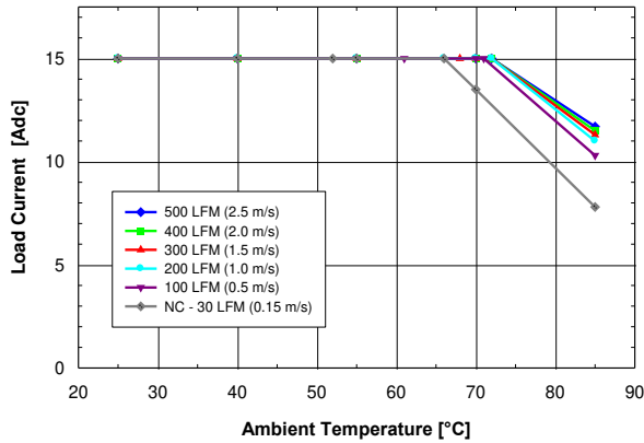
Figure 1. Available load current vs. ambient air temperature and airflow rates for SSQE48T15033 converter mounted vertically with air flowing from pin 1 to pin 3, V_{in} = 48 V . Note: NC – Natural convection
