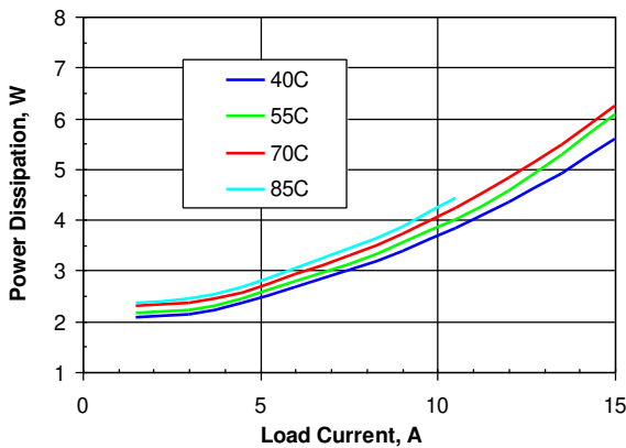
Figure 5. Power dissipation vs. load current and ambient temperature for SSQE48T15033 converter mounted vertically with V_{in} = 48 V and air flowing from pin 1 to pin 3 at a rate of 200 LFM (1.0 m/s)
