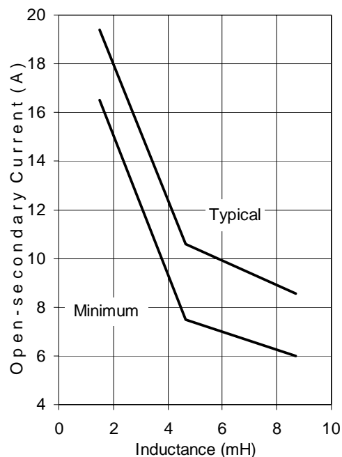
Fig.10 - Self-clamp Avalanche Current vs Inductance @ 150°C
