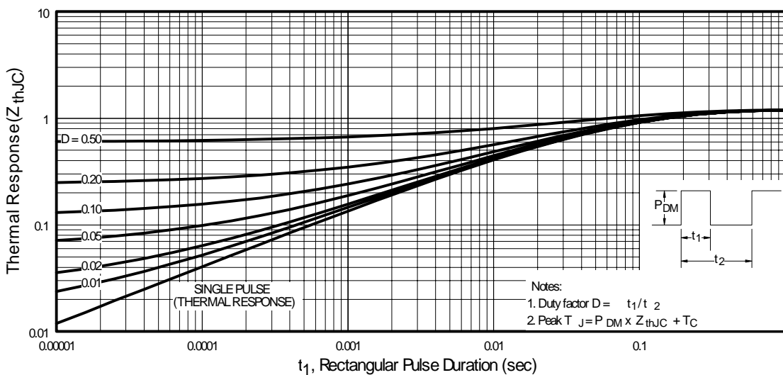
Fig.11 - Transient Thermal Impedance, Junction-to-Case
