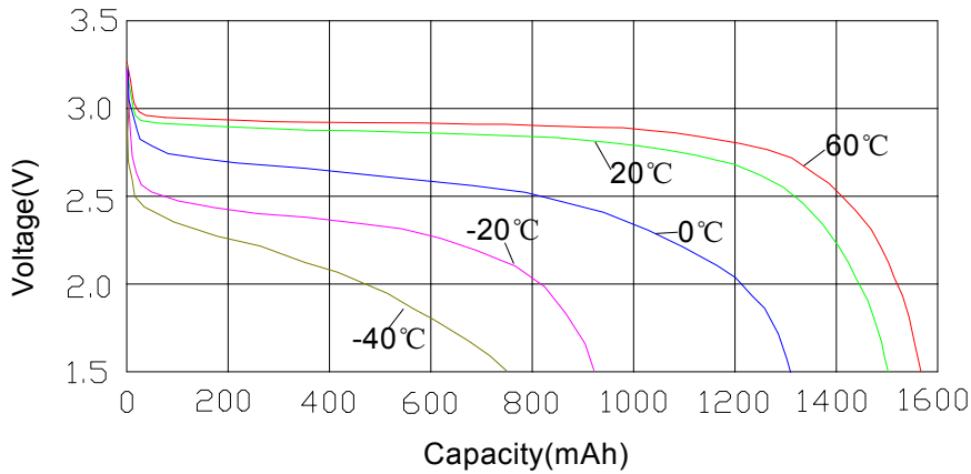
Temperature characteristics(20mA)
