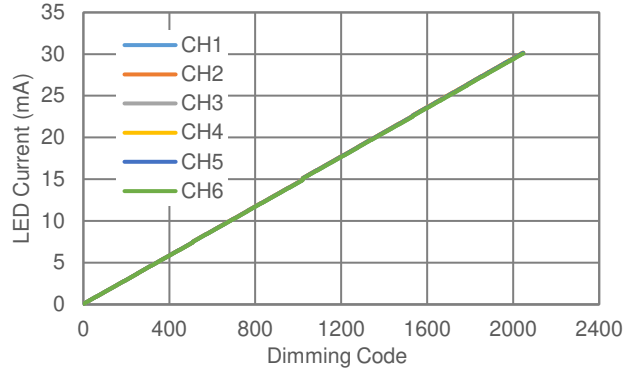
LED Current vs. Current Ratio Code (11 bits, Linear)
