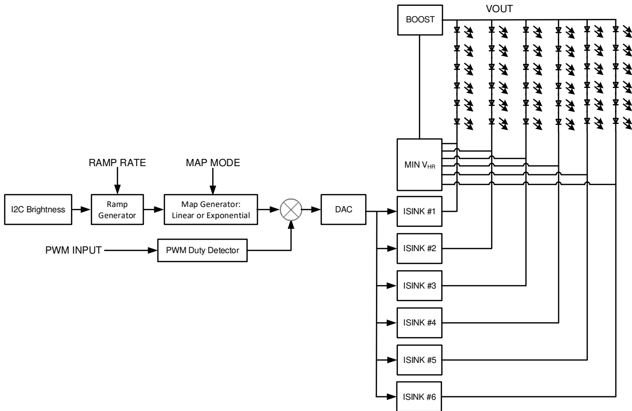
Figure 4. I 2 C and PWM Dimming Scheme
