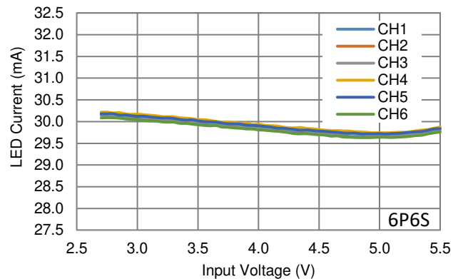
LED Current Line Regulation
