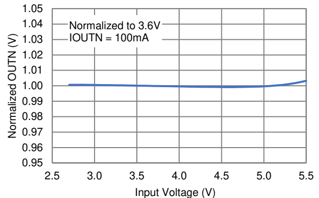
OUTN Line Regulation
