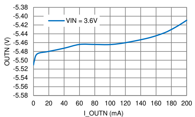
OUTN Load Regulation
