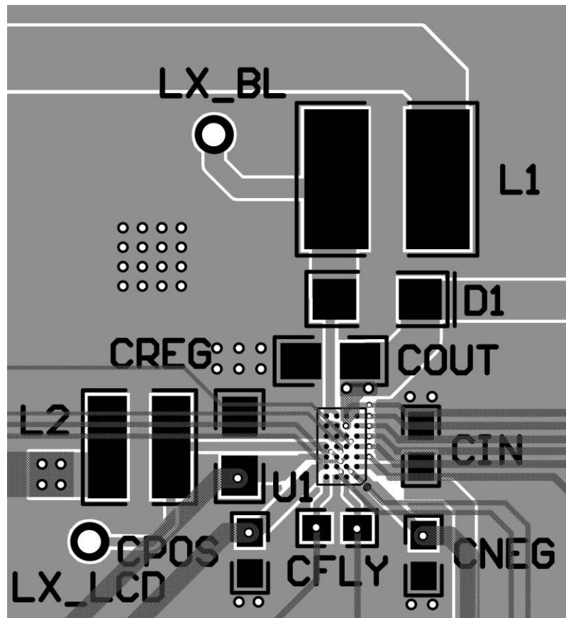
Figure 8. Recommended PCB Layout
