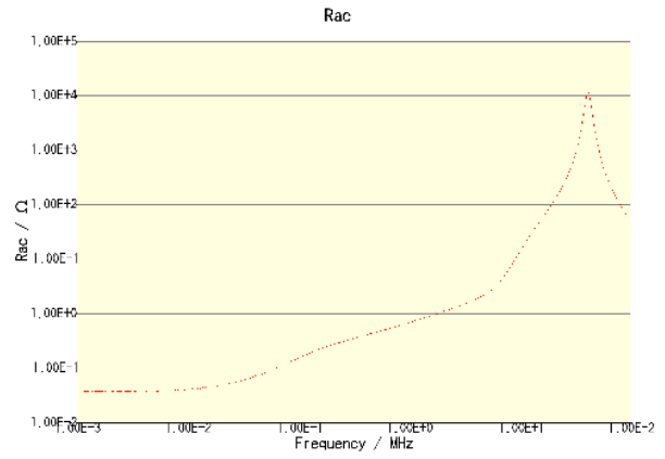
CLF12555T-6R8N-CA
