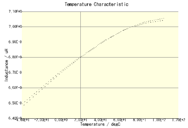
CLF12555T-6R8N-CA(DC = 0A)
