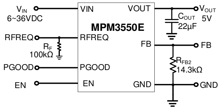
Figure 10: Typical Application Circuit with 5V Output
