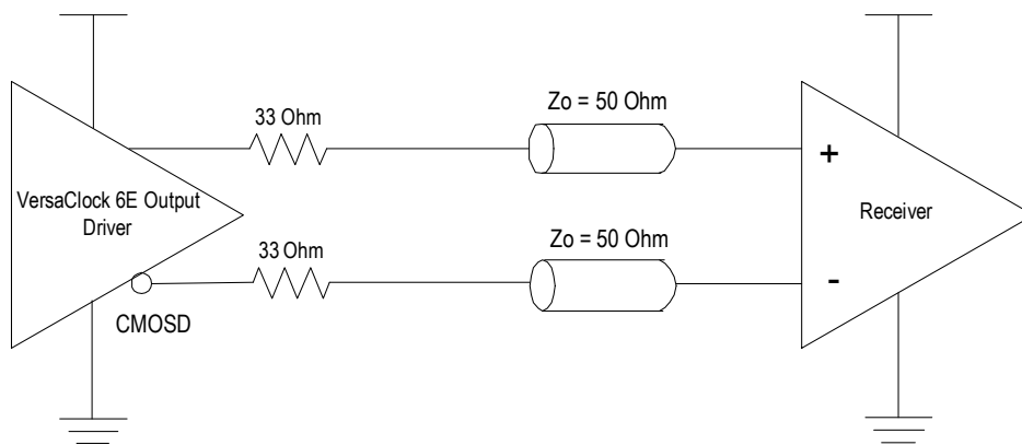
Figure 21. LVCMOS Termination
