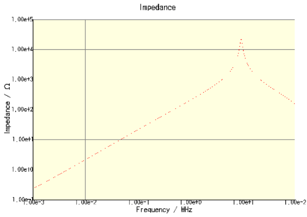
CLF6045T-330M-CA
