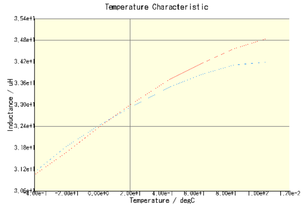
CLF6045T-330M-CA(DC = 0A)
