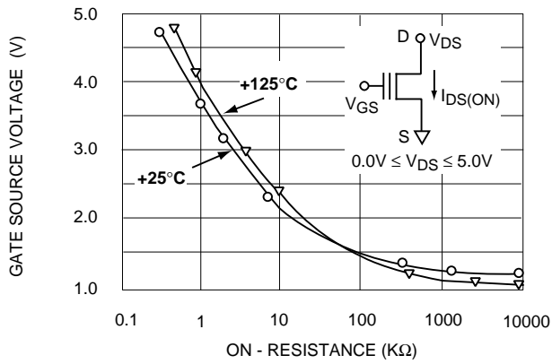
GATE SOURCE VOLTAGE vs. ON - RESISTANCE
