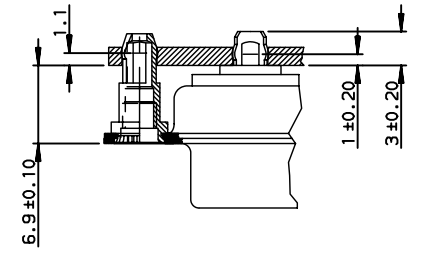
DETAIL OF PRESS FIT
