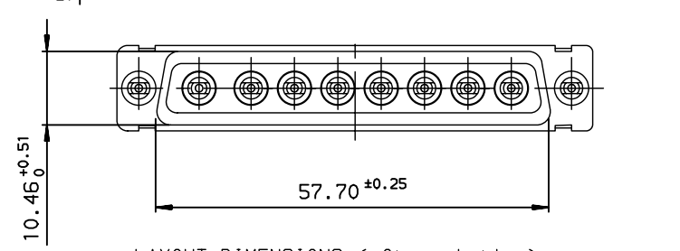
LAYOUT DIMENSIONS (after plating) CONNECTOR SIDE VIEW
