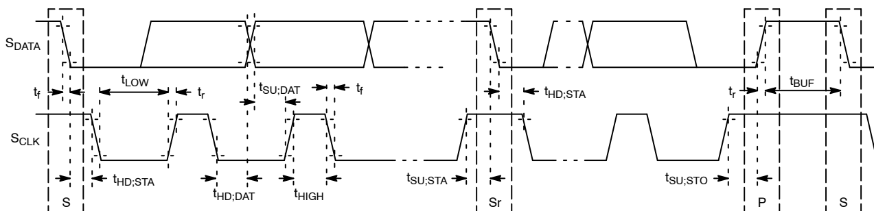
Figure 28. Two-Wire Serial Bus Timing Parameters
