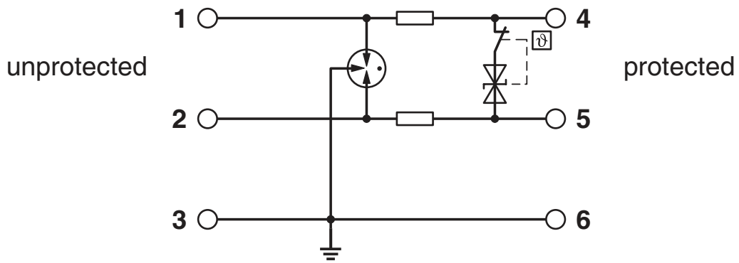
Circuit diagram
