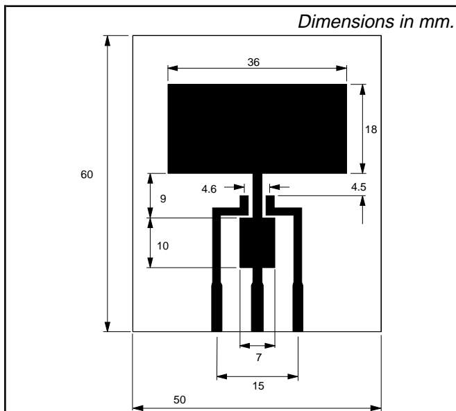
Fig.19. PCB for thermal resistance and power rating. PCB: FR4 epoxy glass (1.6 mm thick), copper laminate (35 \mu m thick).
