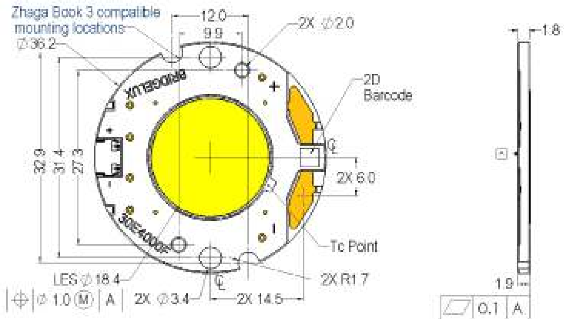
Figure 24: Drawing for Vero 18 LED Array
