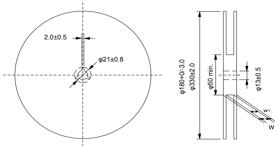
Fig.3 Taping Diagram
