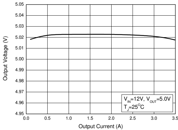
Figure 10. Load Regulation
