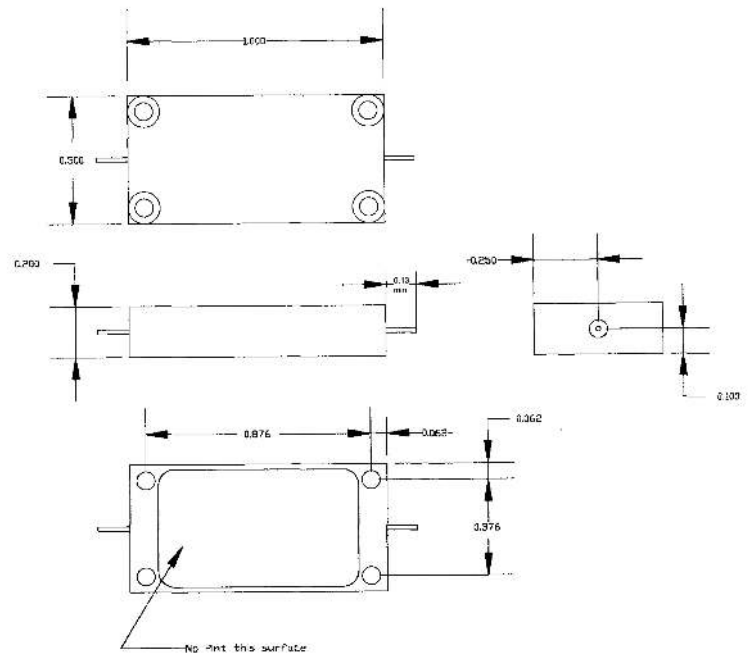
Outline Drawing:
