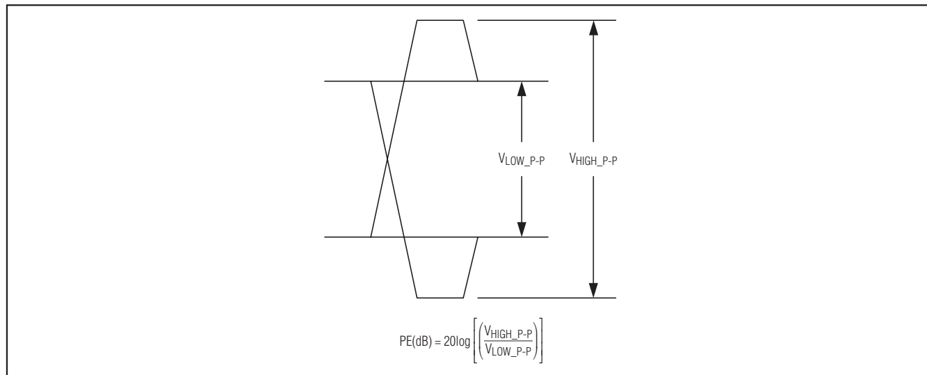
Figure 1. Output Preemphasis
