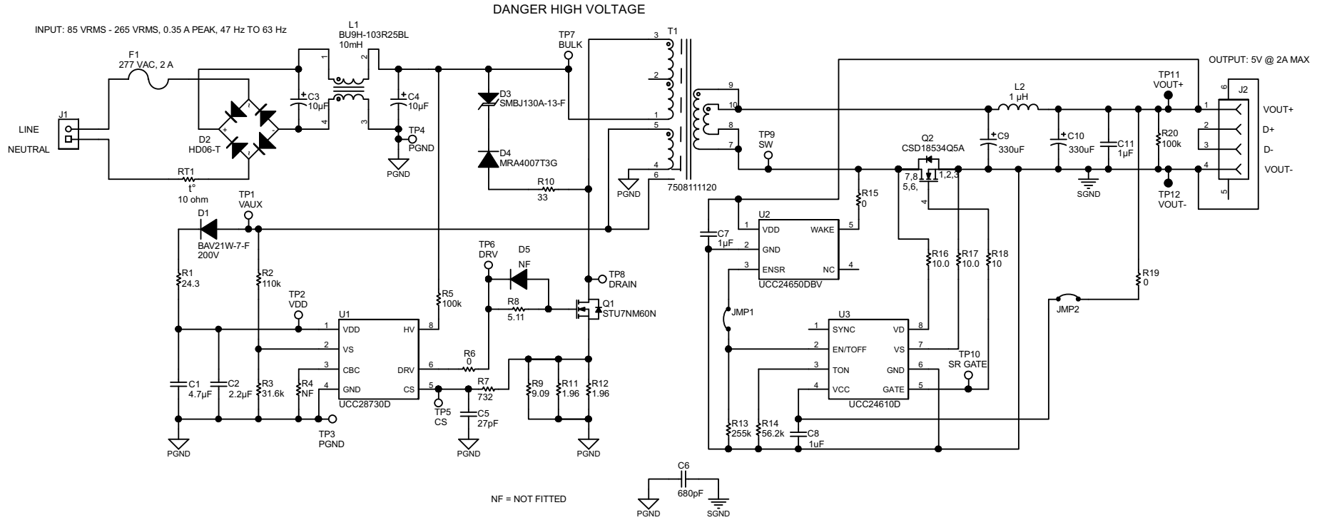
Figure 1. UCC28730EVM-552 Schematic
