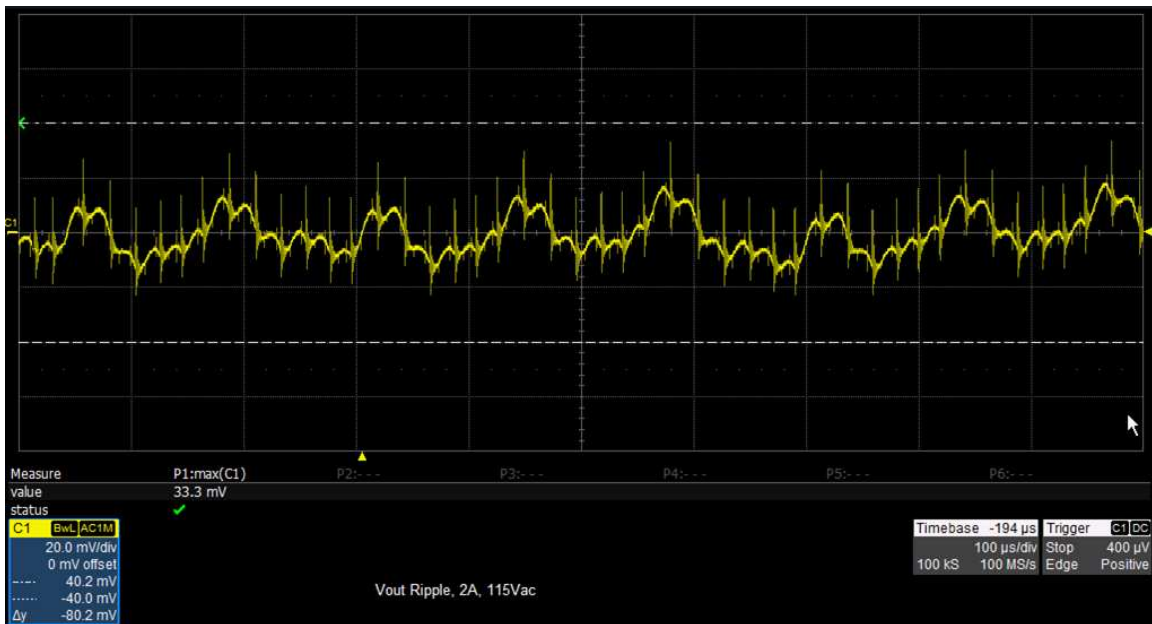
Figure 11. Output Ripple
