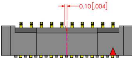
FINAL X AXIS LINEAR MISALIGNMENT
