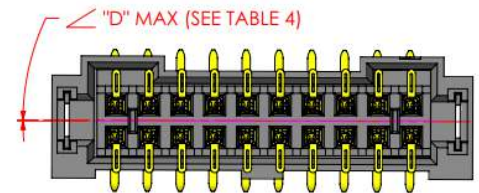
FINAL Z AXIS ANGULAR MISALIGNMENT
