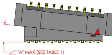
INITIAL Y AXIS ANGULAR MISALIGNMENT
