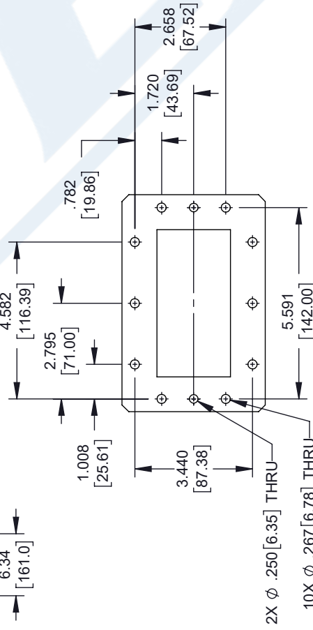
DETAIL A
