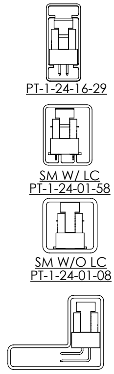
FIG 7 PACKAGING VIEWS
