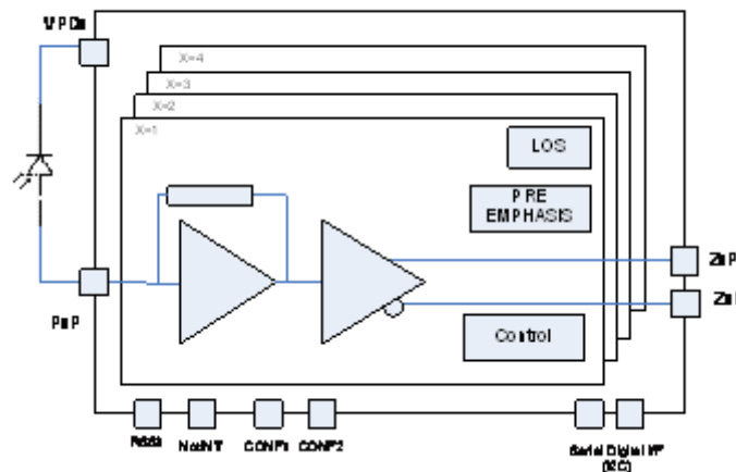
Figure 1: Device diagram
