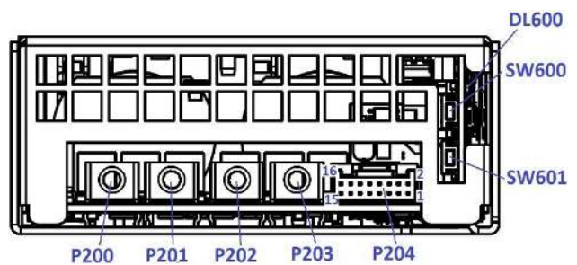
Figure 7. Rear View - MCC750-1T24-PC / MCC750-1T48-PC Models
