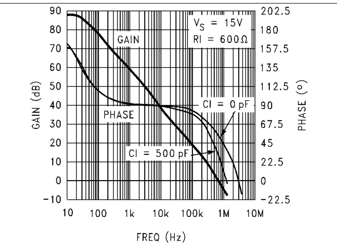
Figure 38. Gain and Phase vs Capacitive Load
