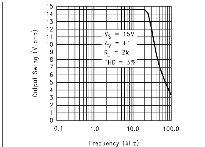
Figure 37. Maximum Output Swing vs Frequency
