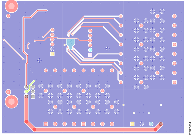
Figure 14. EV-ADGS1414DSDZ Bottom Layer
