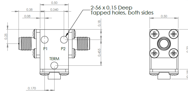
D313841 Dimensions
