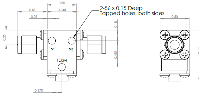
D313841-3 Dimensions
