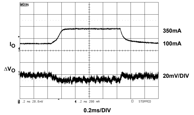
FIGURE 8. TRANSIENT RESPONSE
