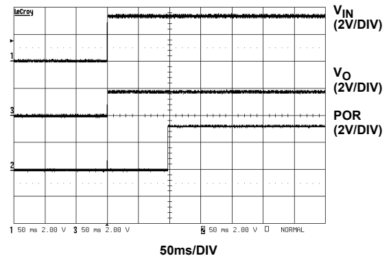
FIGURE 6. START-UP 2
