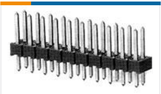
TE Part #5-146252-1 02 MODII HDR DRST B/A .100 LF
