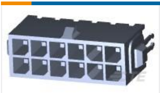
TE Part #4-794682-2 12P MICRO MNL ASSY,VRT,THRU,LF
