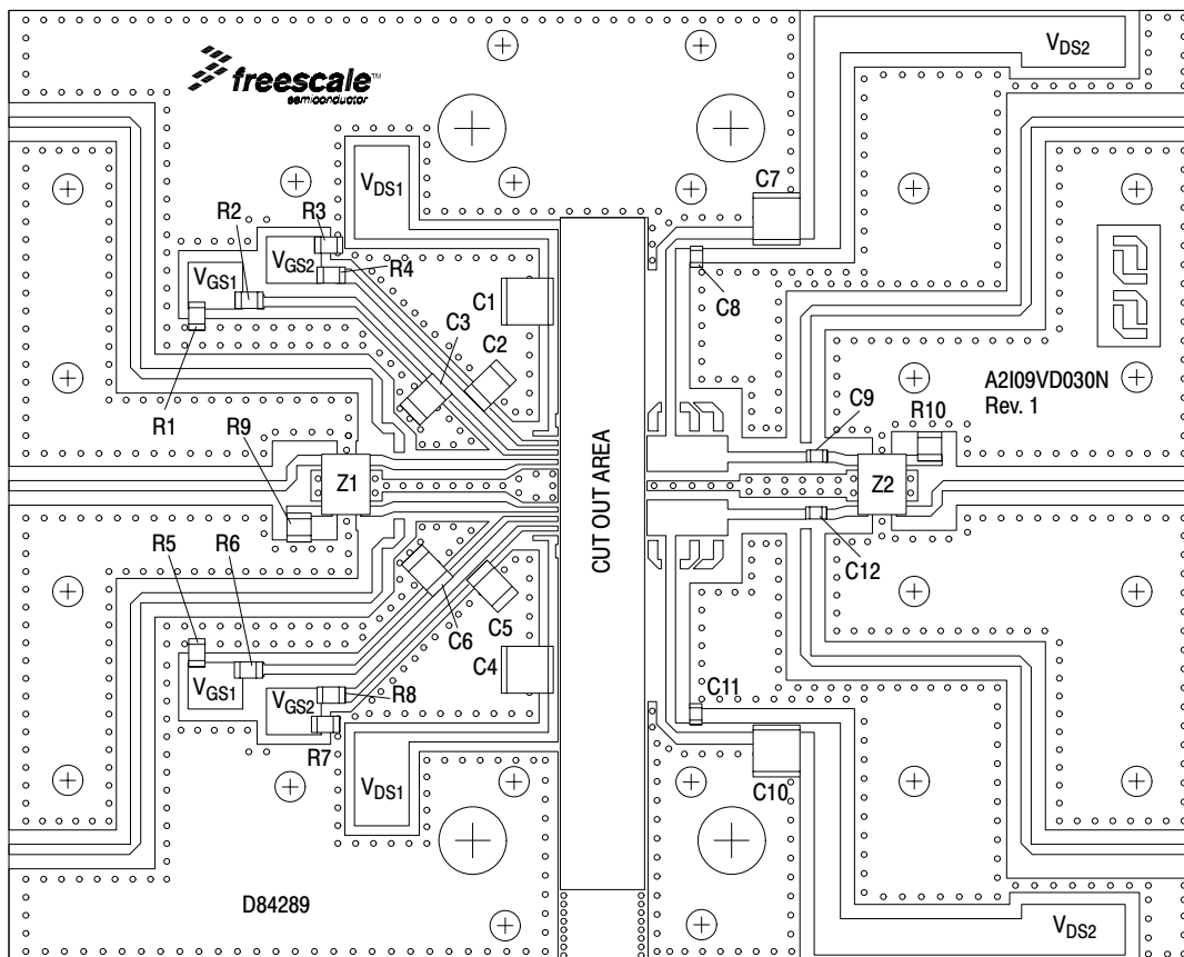
Figure 17. A2109VD030N Test Circuit Component Layout – 728–768 MHz
