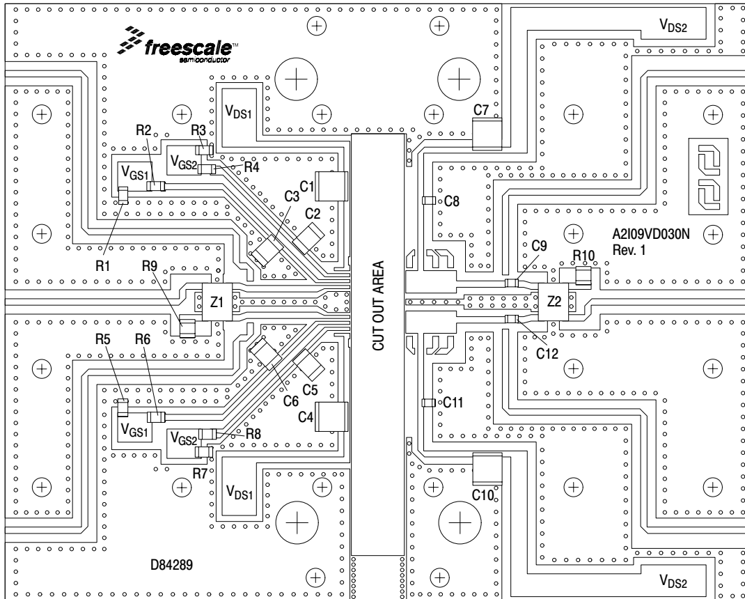
Figure 3. A2109VD030N Test Circuit Component Layout – 920–960 MHz
