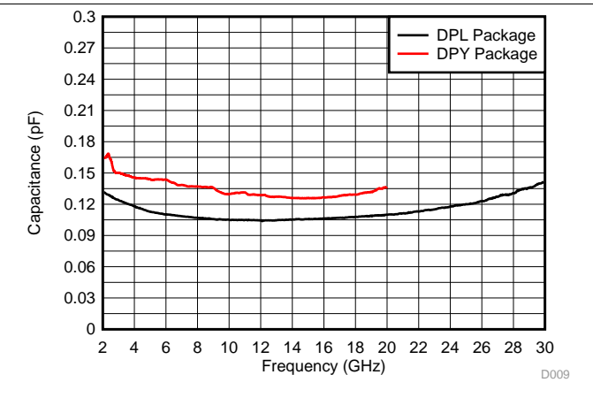
Figure 10. Capacitance vs. Frequency
