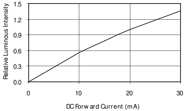
Figure 3. Relative Iv vs. Forward Current
