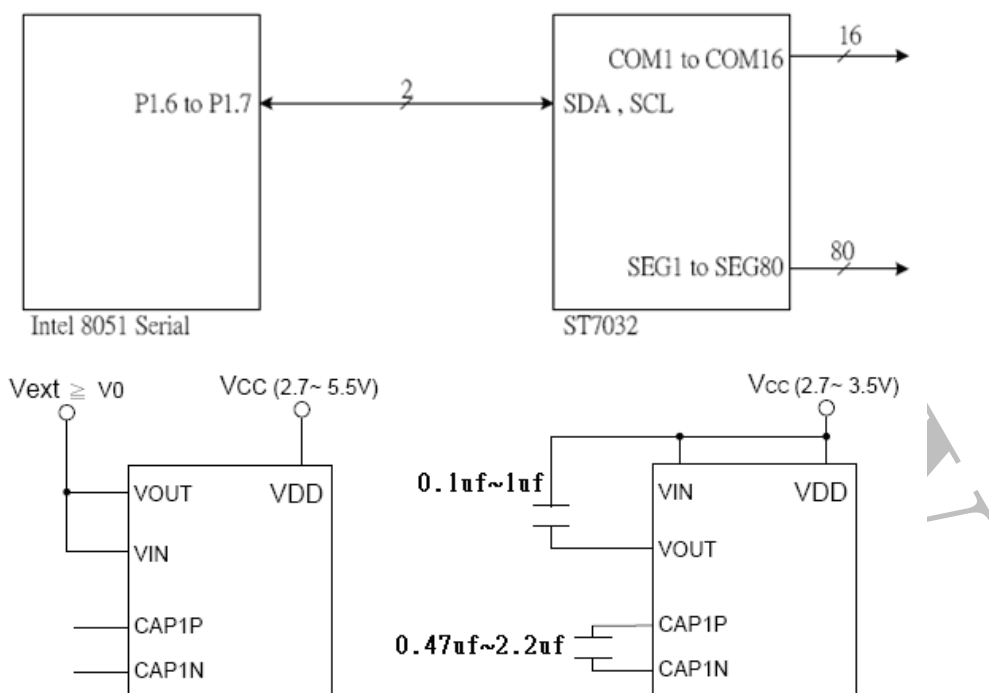
Intel 8051 interface( I 2 C )
