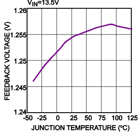
Feedback Voltage vs. Junction Temperature V_{IN}=13.5V
