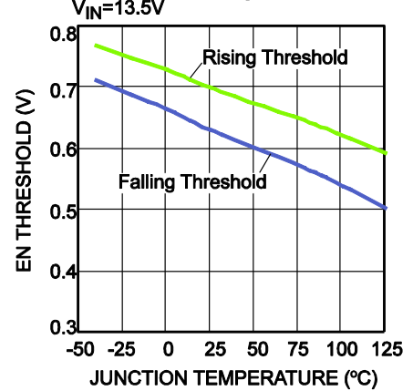
EN Threshold vs. Junction Temperature V_{IN}=13.5V
