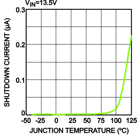
Shutdown Current vs. Junction Temperature V_{IN}=13.5V
