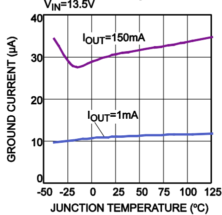
GND Current vs. Junction Temperature V_{IN}=13.5V
