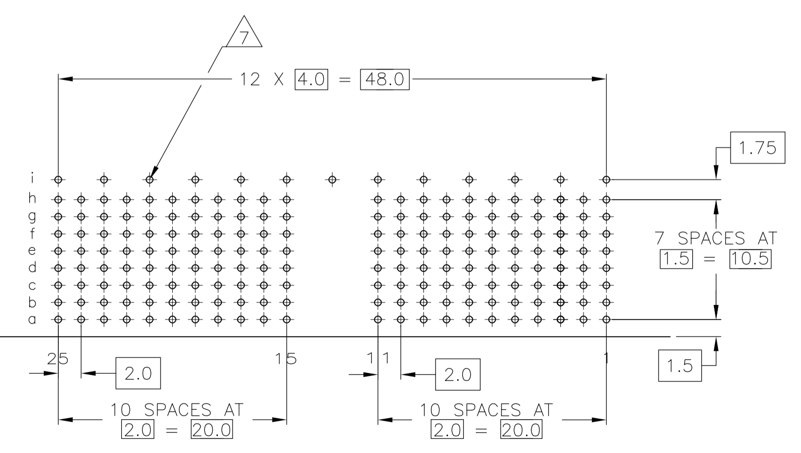
EDGE OF P.C. BOARD RECOMMENDED PCB-HOLE LAYOUT COMPONENT SIDE SHOWN SCALE 3:1
