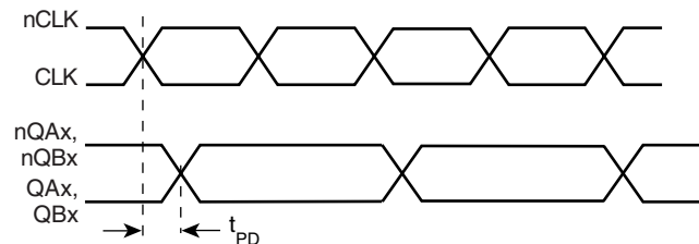
PROPAGATION DELAY
