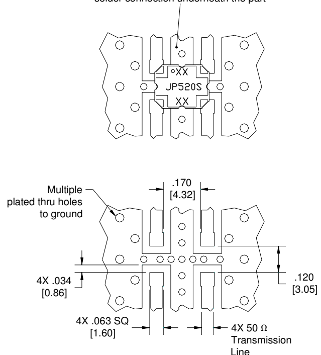
Dimensions are in Inches [Millimeters] JP520S Mounting Footprint
