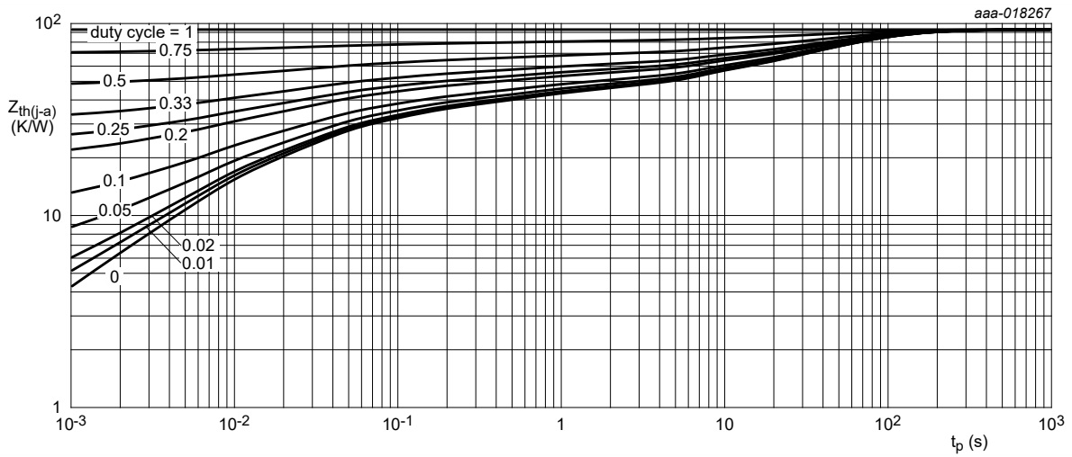
FR4 PCB, mounting pad for anode and cathode 1\text{ cm}^2 each
